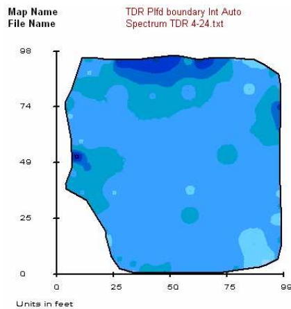
Figure 5. Interpolated map for a TDR 300 soil moisture meter
